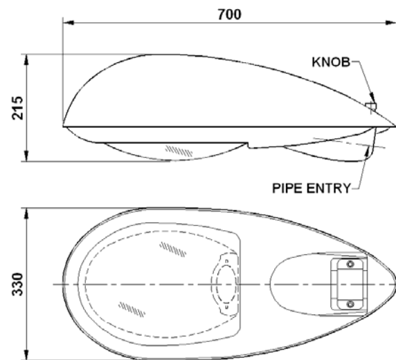
NOMINAL DIMENSIONS IN mm Tolerance +/-5
